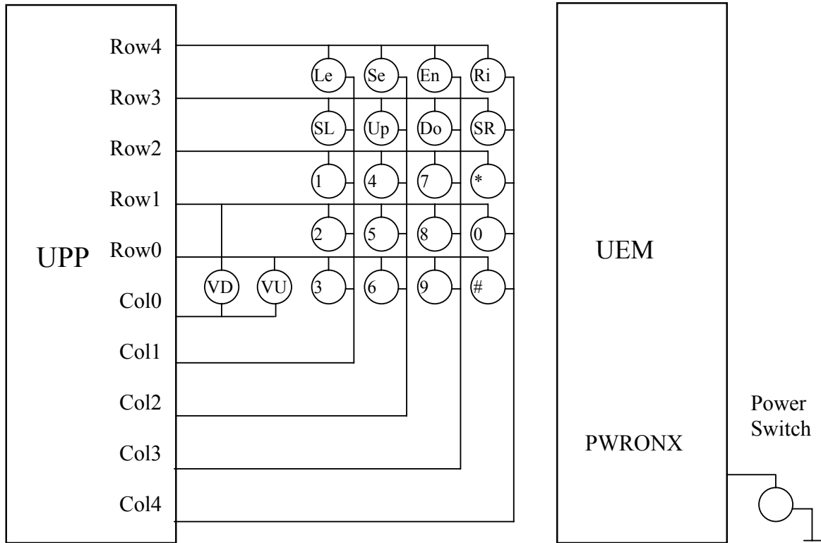
Figure 25: Keyboard matrix connections.
