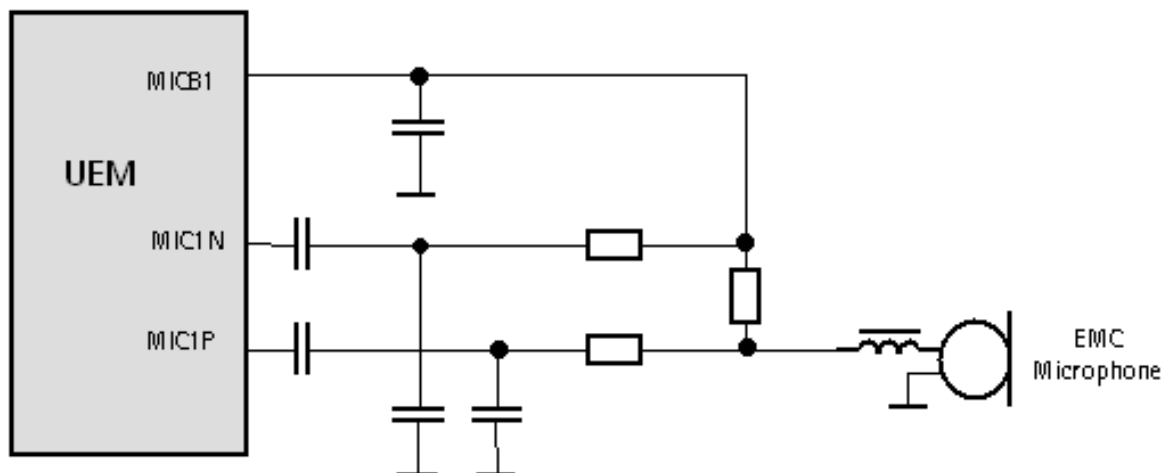
Figure 13: Internal microphone
