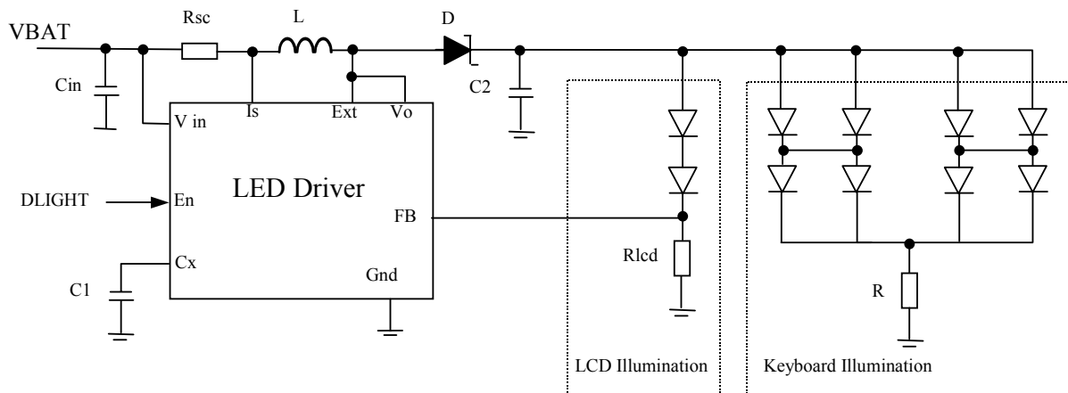
Figure 27: LCD & keypad illumination.
