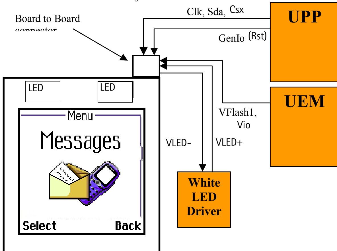
Figure 26: LCD connections.
