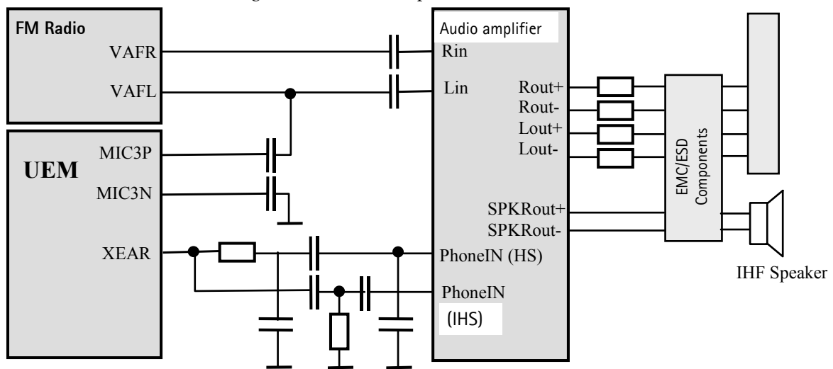
Figure 11: External Earphone & IHF Connections
