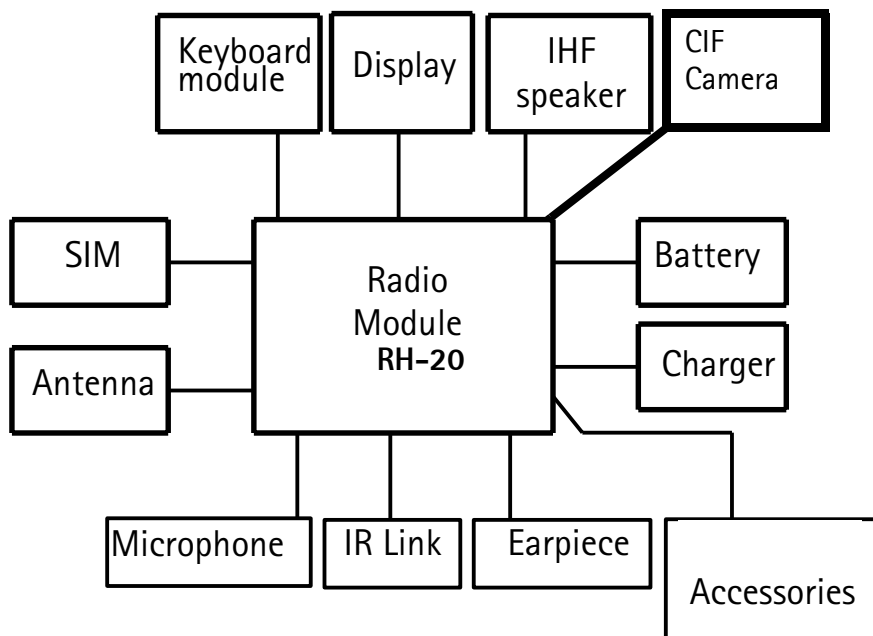
Figure 1: Interconnection diagram
