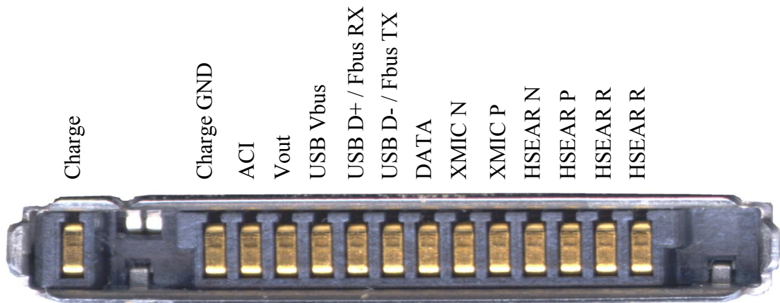
Figure 29: Pop-Port connections.
