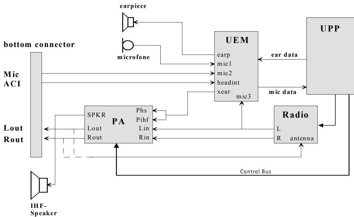
Figure 17: Audio block diagram RH-20
