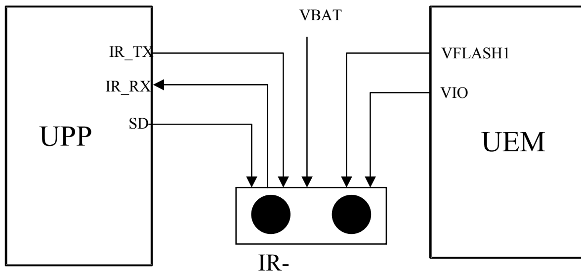
Figure 28: IR module connections.
