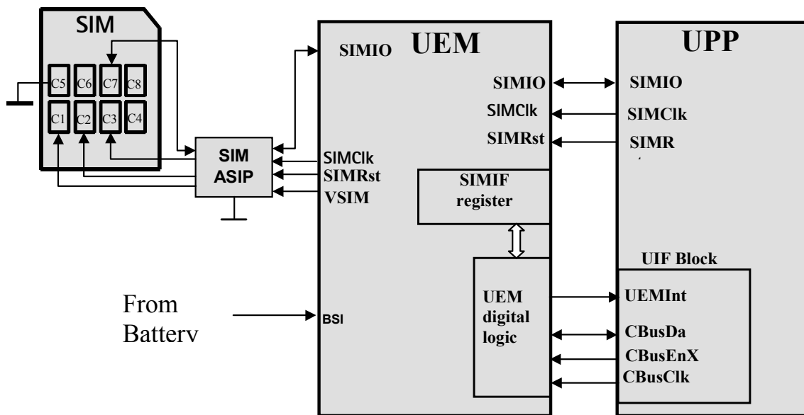
Figure 8: SIM interface RH-20
