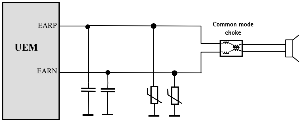
Figure 14: Internal speaker
